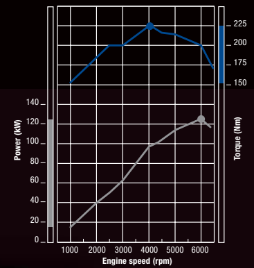
2.4L MIVEC DOHC Engine
